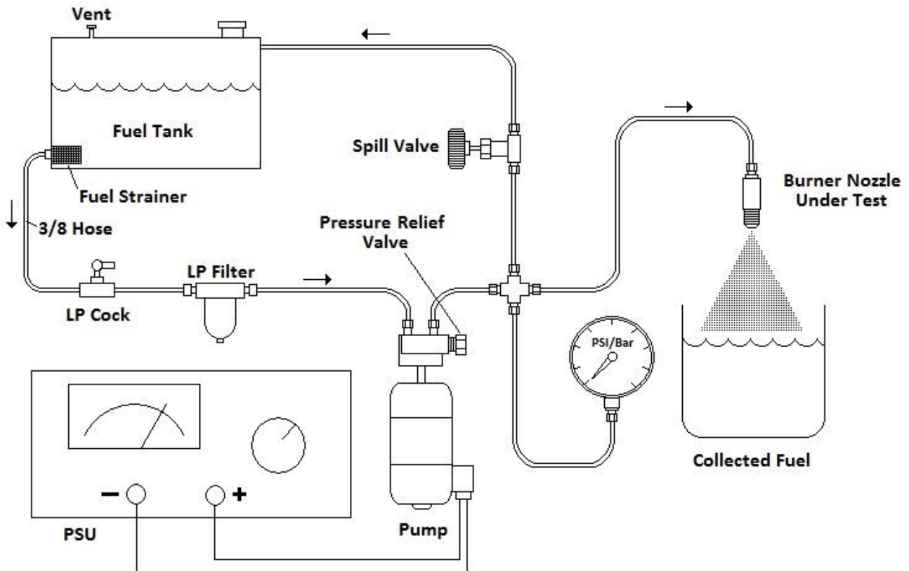
Simple burner test rig
